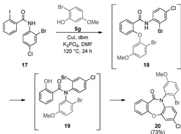
Scheme 6. In situ trapping of Smiles rearrangement intermediate 19 .
